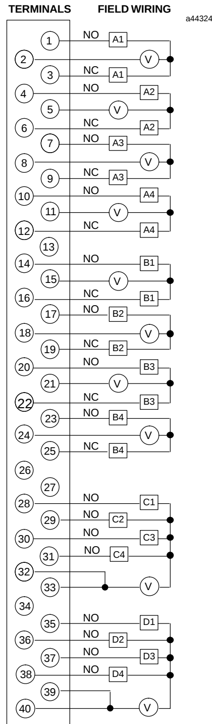
Figure 2. Field Wiring Connections
